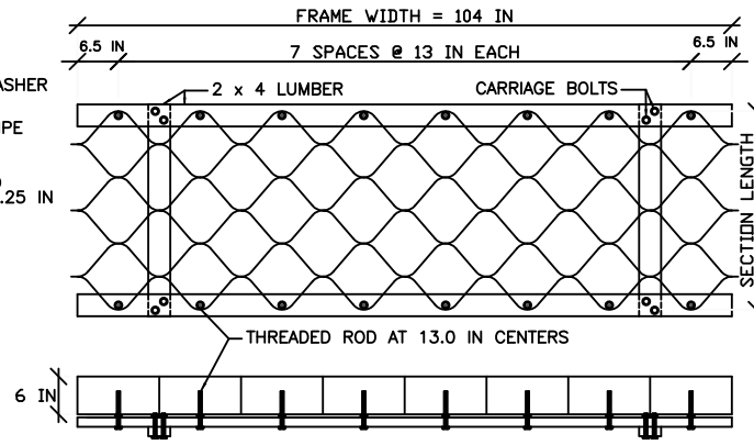
SIDE VIEW - UPSIDE DOWN FOR EXPANSION OF GEOWEB SECTION
